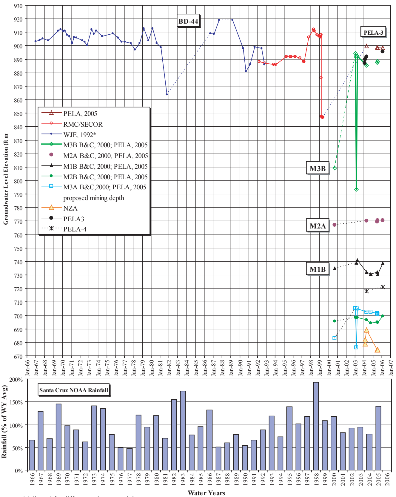
Groundwater Level Hydrographs for Wells BD-44, M1B, M2A, M2B, M3A, M3B, NZA, and PELA-3 and -4
